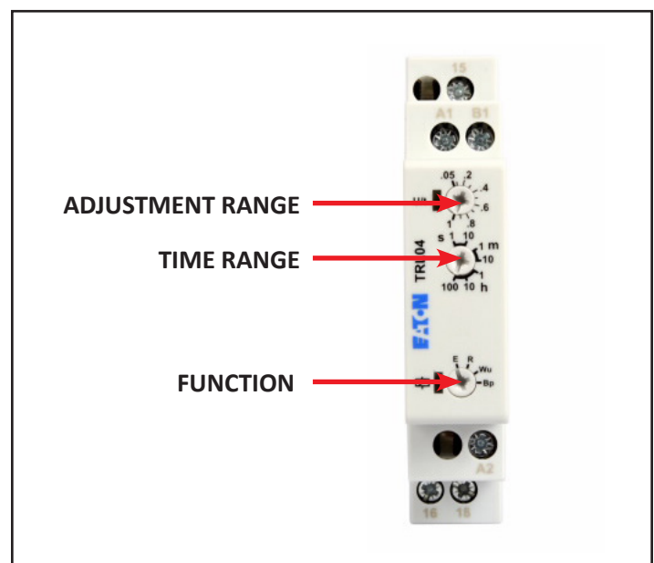
Fig. 35.2: Eaton TRL04 Setting Identification
