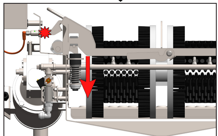
Fig. 35.1: Grate triggering Prox Switch, shown on BLX-800R
